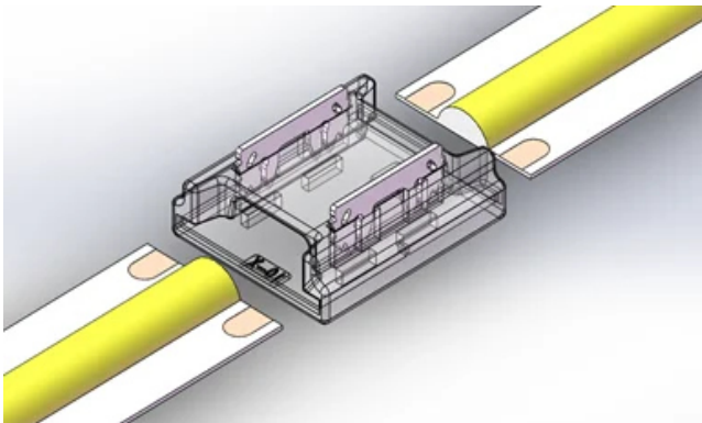
Push the LED Strip into the Connector
