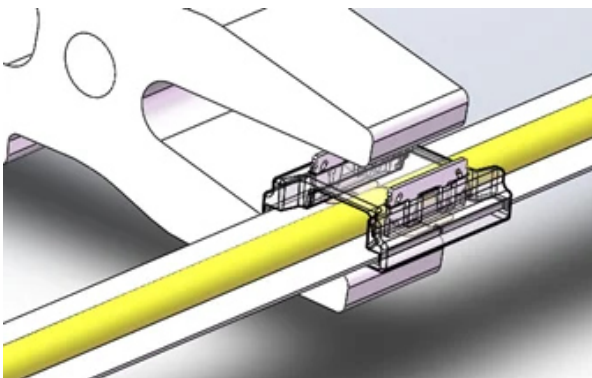
Use pliers to clamp the terminals to the level of the plastic surface, clamping from both sides to ensure that all terminals connect electrically
