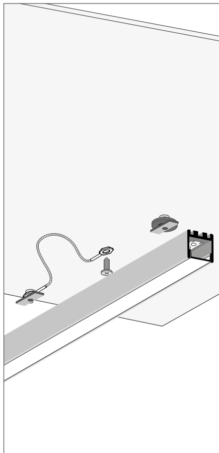
a) Installation with the ZM-1 security wire (secured directly to the mounting surface) - p. 2
