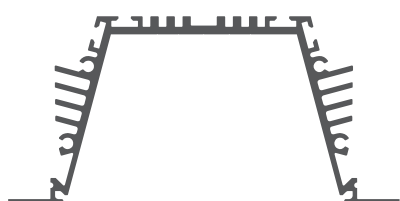
Extrusion (A)
